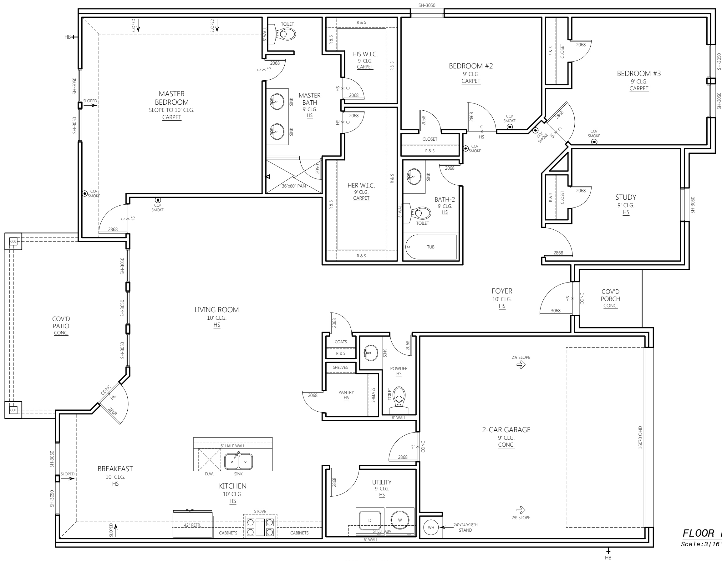
FLOOR PLAN
